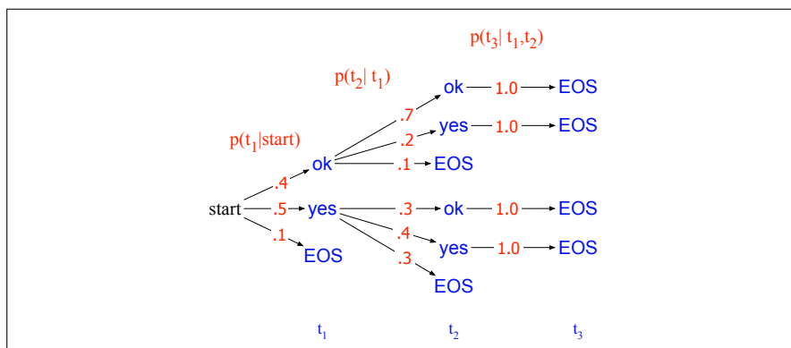
Figure 13.7 A search tree for generating the target string T = t_1, t_2, \dots from vocabulary V = \{\text{yes}, \text{ok}, \text{<s>}\} , showing the probability of generating each token from that state. Greedy search chooses yes followed by yes , instead of the globally most probable sequence ok ok .
