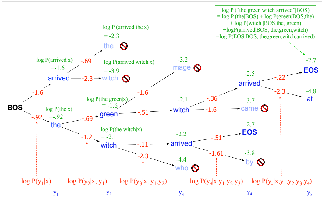
Figure 13.9 Scoring for beam search decoding with a beam width of k = 2 . We maintain the log probability of each hypothesis in the beam by incrementally adding the logprob of generating each next token. Only the top k paths are extended to the next step.
