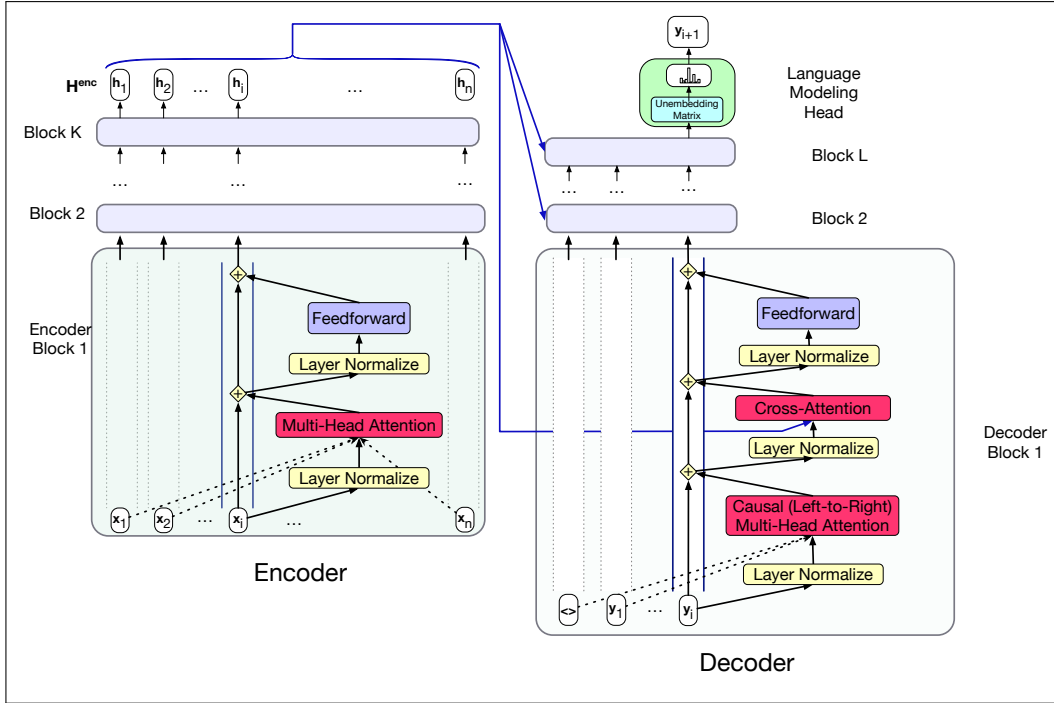
Figure 13.6 The transformer block for the encoder and the decoder, showing the residual stream view. The final output of the encoder \mathbf{H}^{enc} = \mathbf{h}_1, \dots, \mathbf{h}_n is the context used in the decoder. The decoder is a standard transformer except with one extra layer, the cross-attention layer, which takes that encoder output \mathbf{H}^{enc} and uses it to form its K and V inputs.
